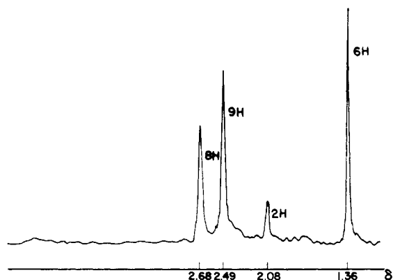
Figure 4. ^1\text{H} nmr spectrum of cation 28 at +27^\circ .
